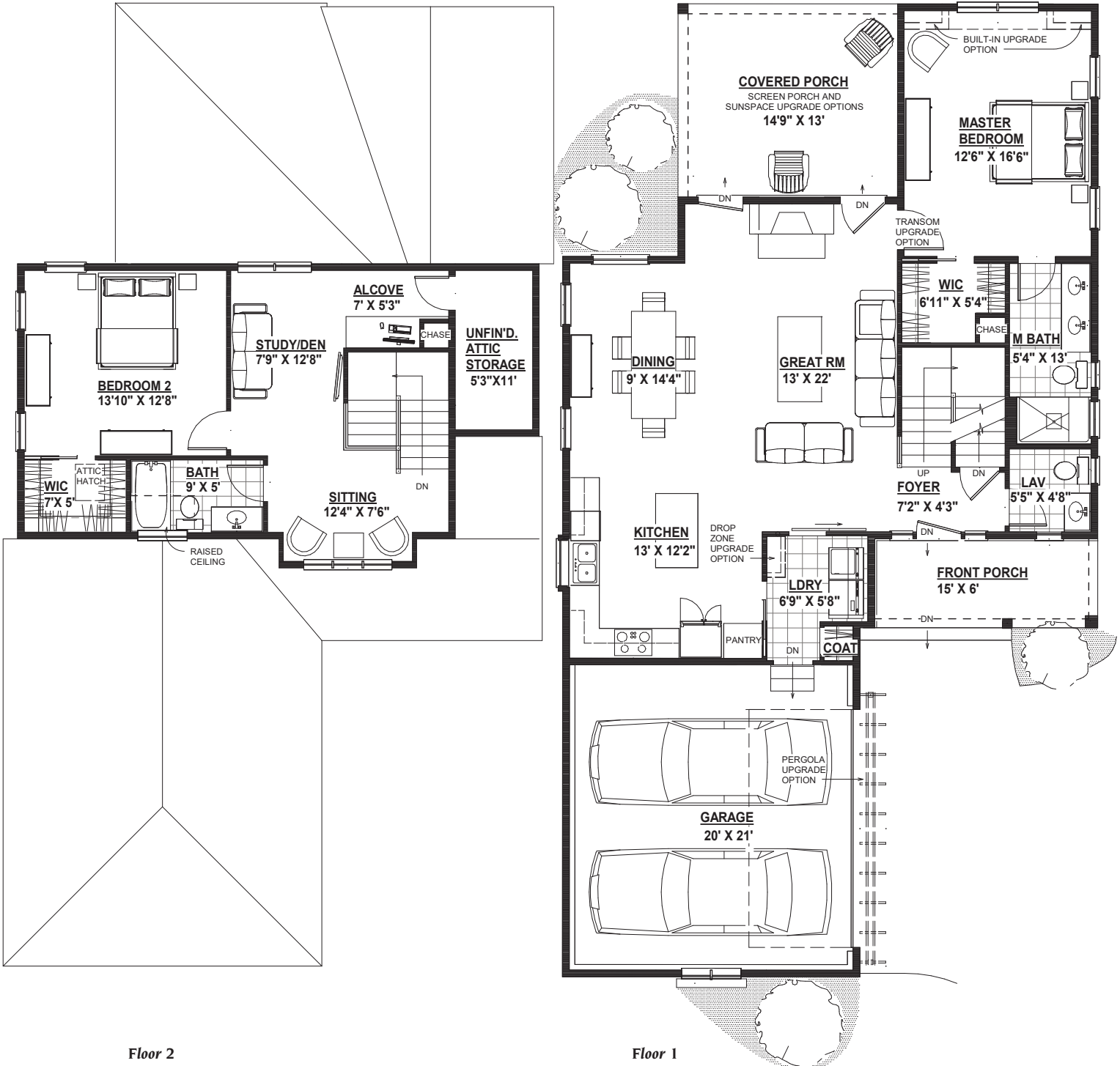
Floor Plan
